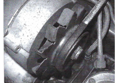
Here you see the correct alternator fan. It turns counterclockwise. Note the direction of the blades so that it will suck-in cooling air from the back of the alternator.
